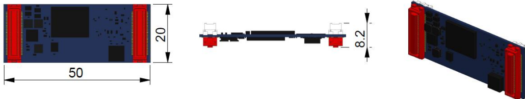
CP400.85 outer dimensions [mm]
